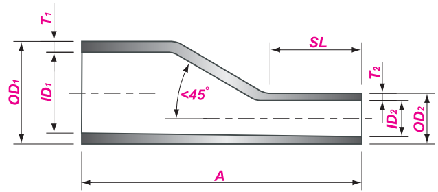
偏心异径短节 Eccentric Swaged Nipple
